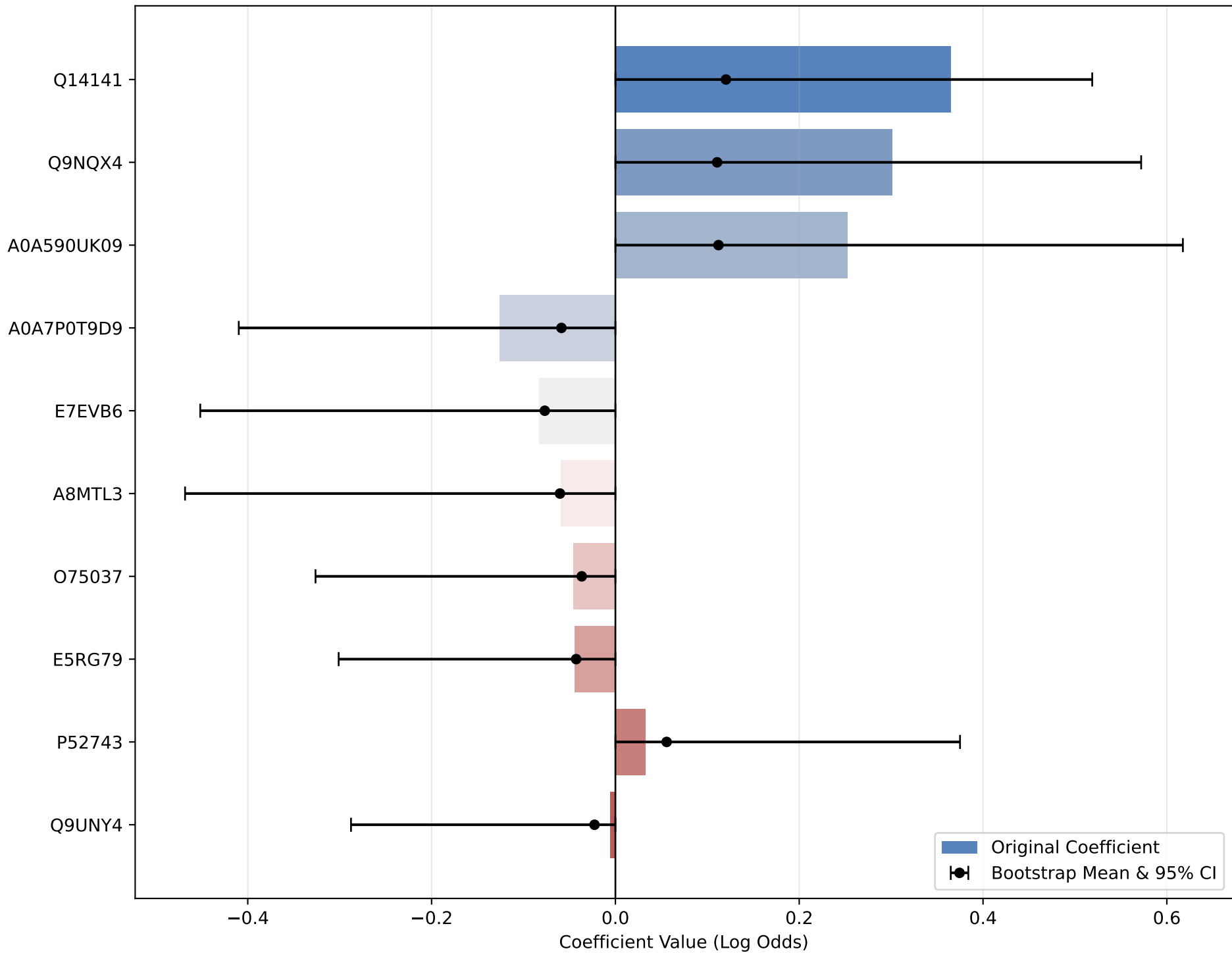
Top 10 Features (Bars = Original, Points/Lines = Bootstrap 95% CI)
